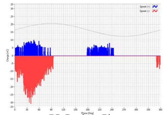
PD Peak vs Phase
