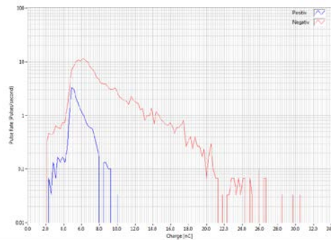
Pulse Height
