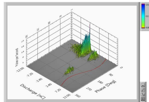
3D PRPD Pattern
