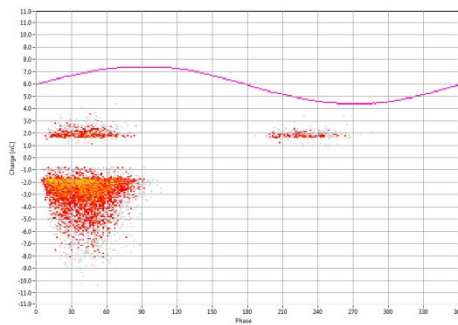
2D PRPD Pattern
