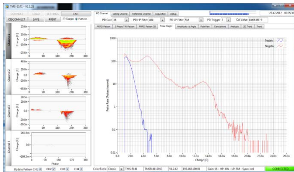
Pulse Height Distribution Pulse Height Distribution
