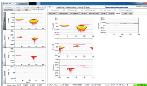
3Phase Cross Analysis
