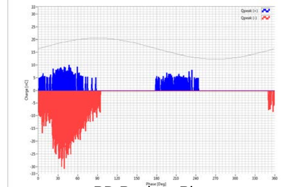
PD Peak vs Phase
