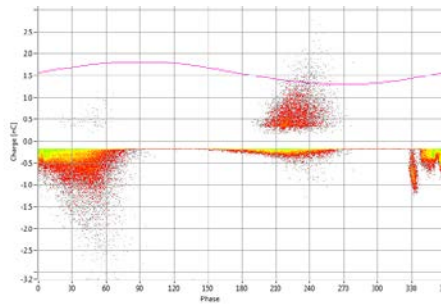
2D PRPD Pattern
