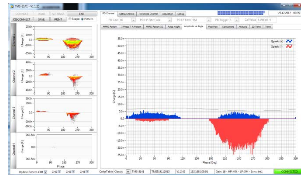
PD Peak vs Phase
