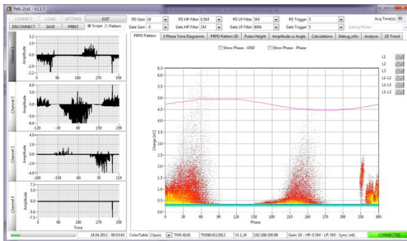
Unipolar PRPD Pattern
