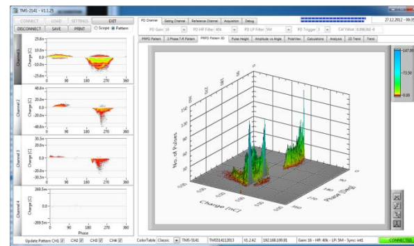
3D PRPD Pattern
