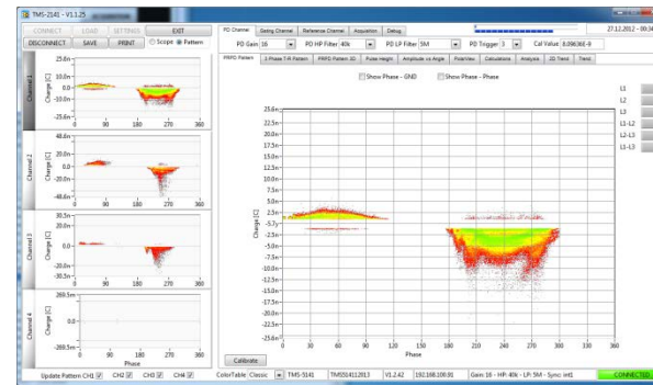
Bipolar PRPD Pattern
