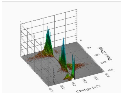
3D PRPD Pattern
